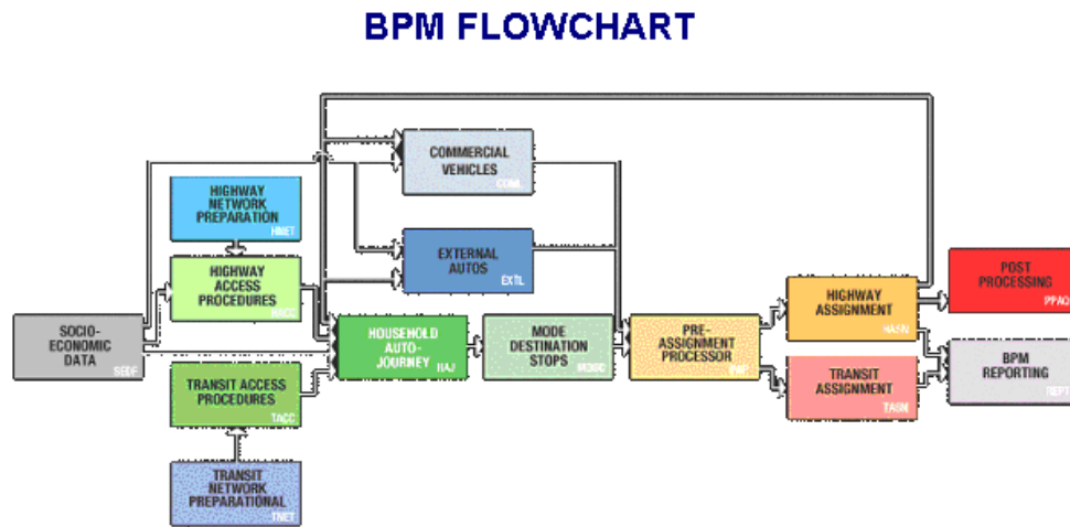
Figure 1: NYBPM Flowchart
