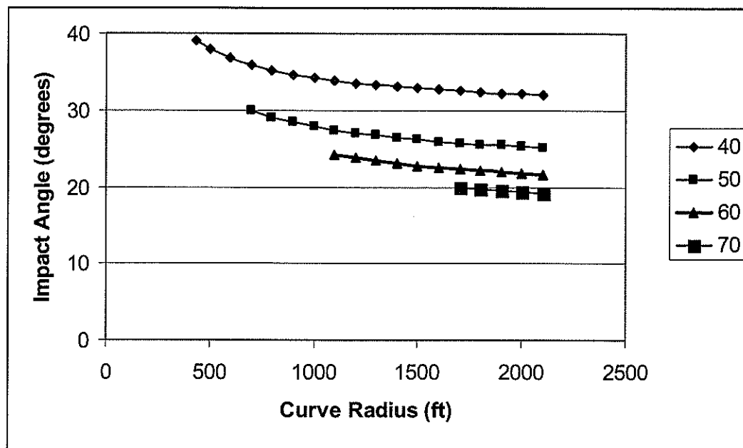
(b) Impact Angles for Maximum Separation Distance of 42 ft.
