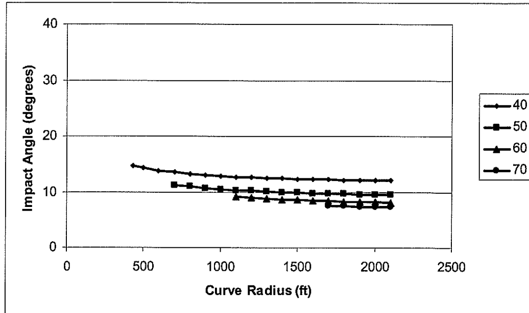
(a) Impact Angles for Maximum Separation Distance of 6 ft.
