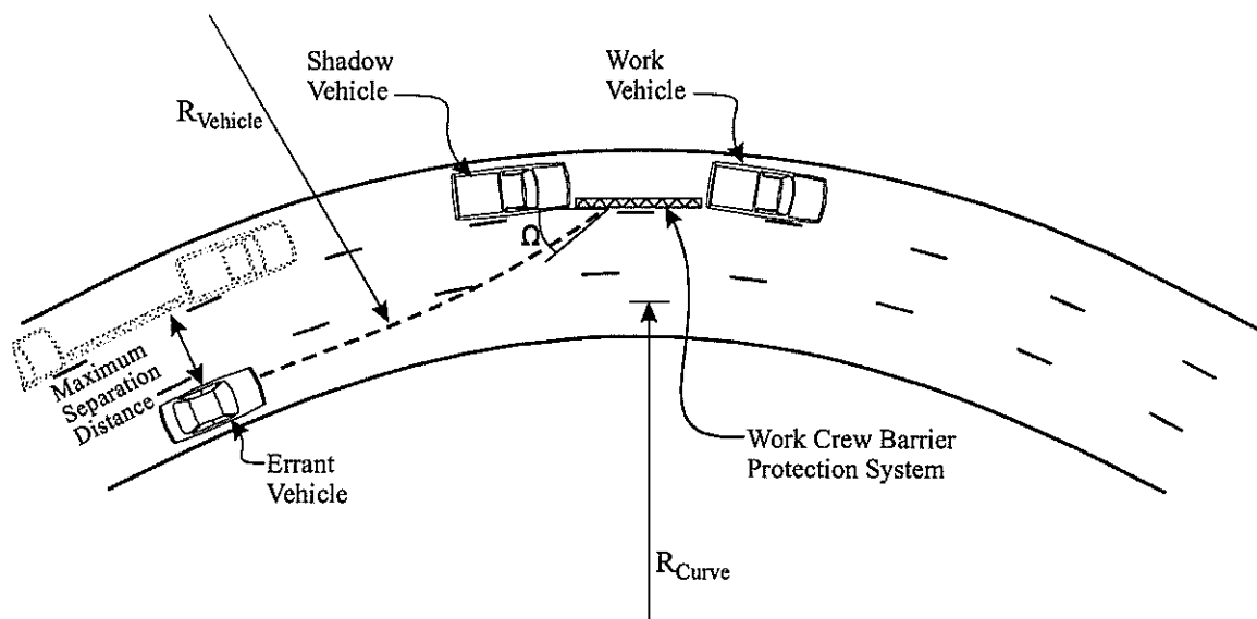
Figure 1. Illustration of Impact Condition on a Horizontal Curve.
