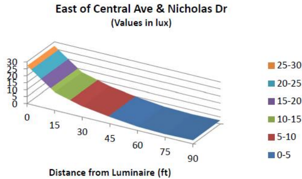
Figure 6. Measured illuminances along the sidewalk at Central Avenue and Nicholas Drive.
