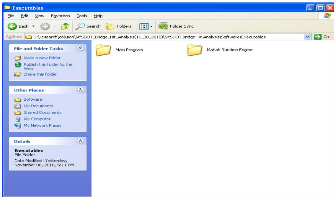
Figure 5-4: Executables Folder
