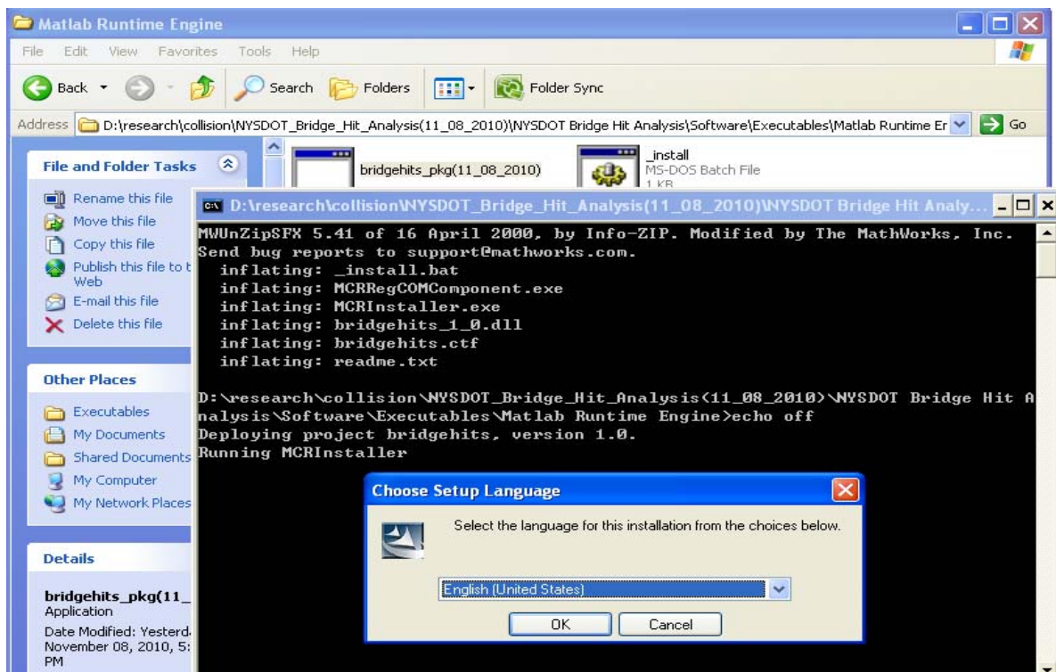
Figure 5-8: Click OK.
