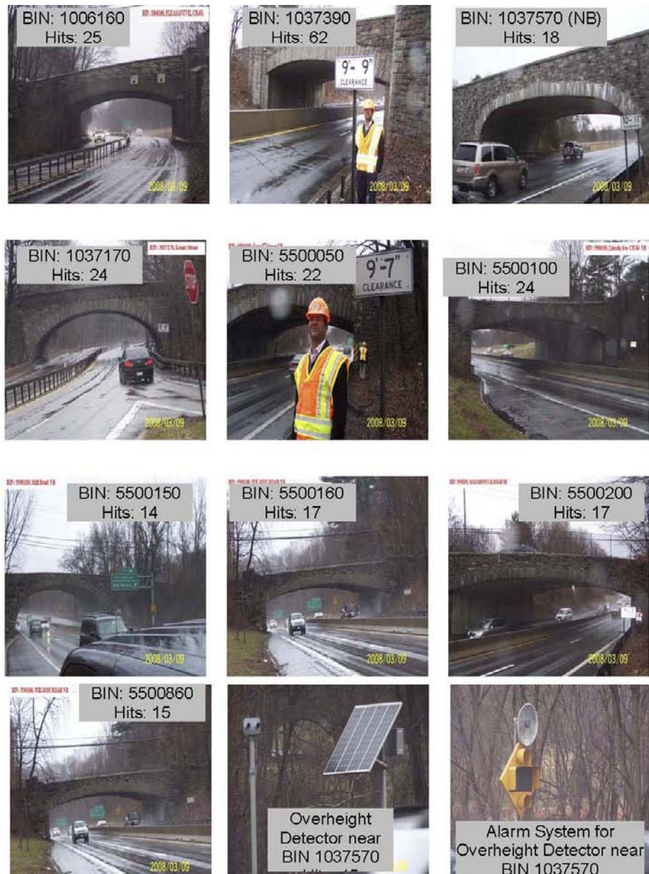
Figure 3-17: Pictures of Most Frequently Hit Bridges in Region 8. Last two pictures show over-height detection system installed near a bridge (system not functional).
