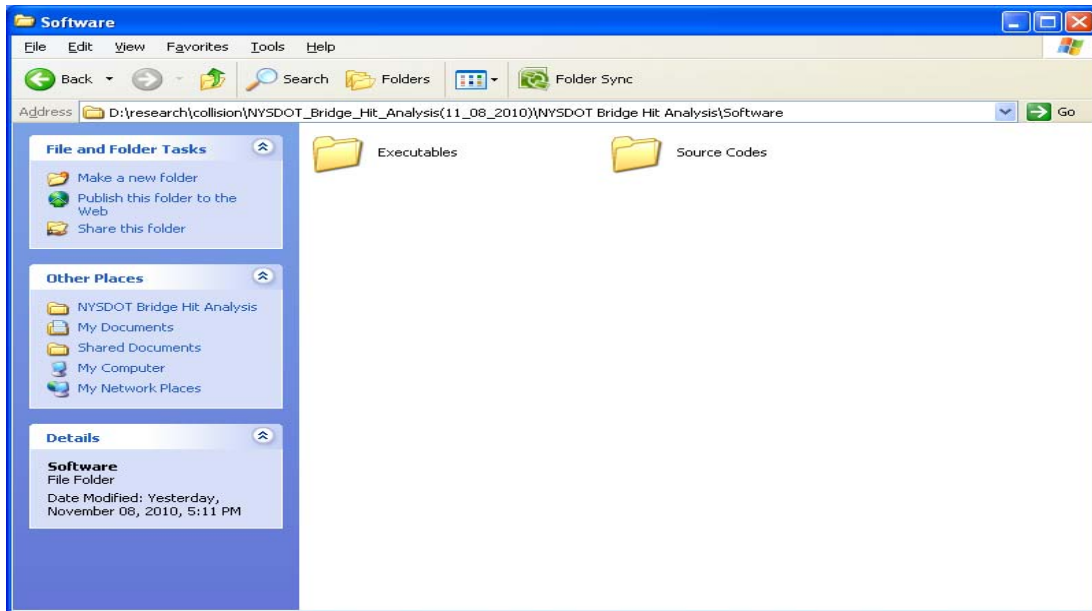
Figure 5-3: Software folder.
