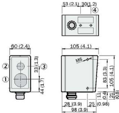
Dimensions HISIC450 in mm (in)
