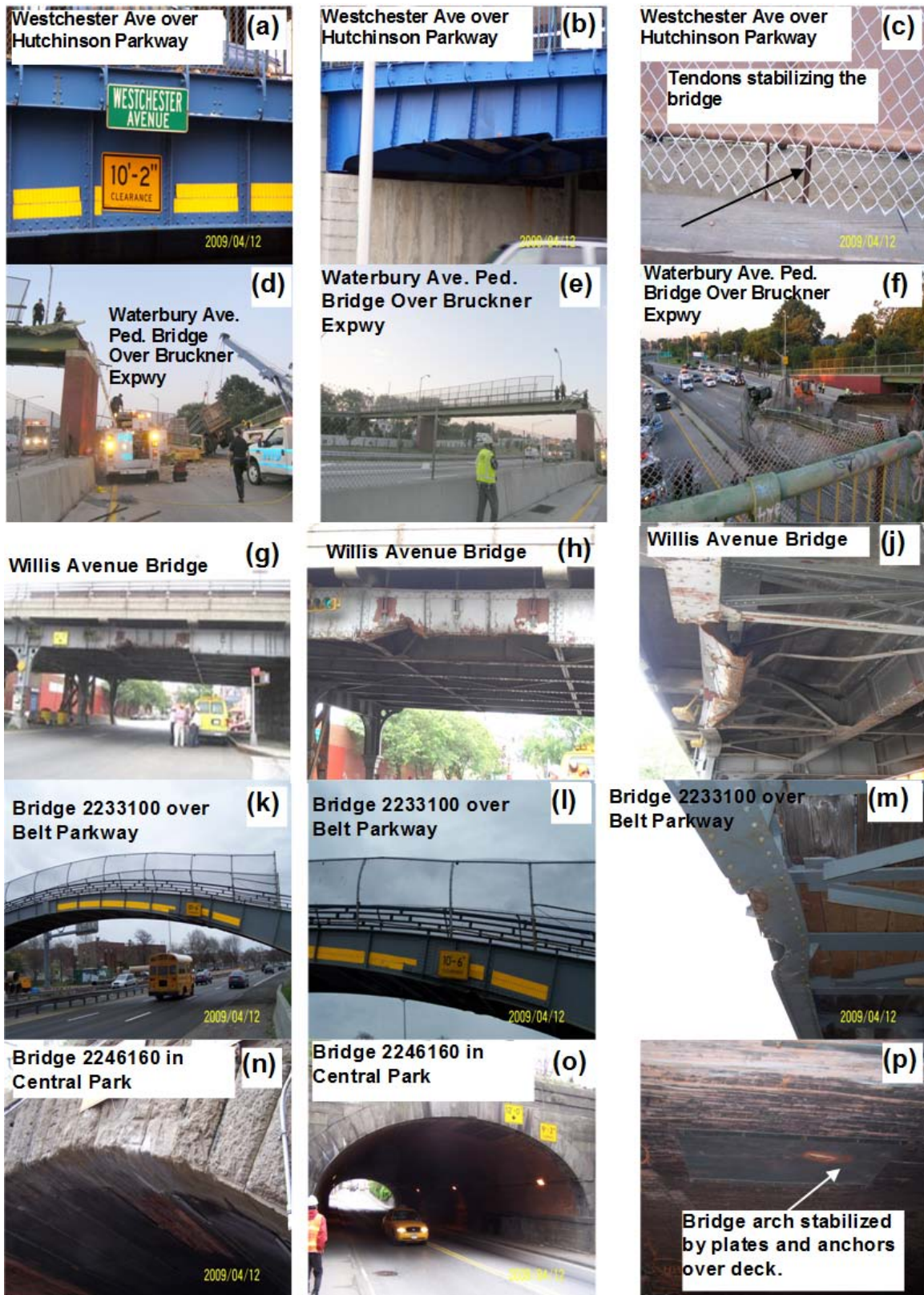
Figure 3-27: Damages to the Bridges in the New York City Area (Region 11)
