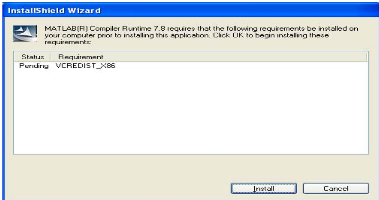
Figure 5-9: Click Install.
