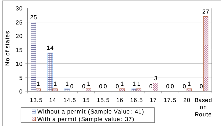
Figure 2-12: Maximum Heights for Vehicles and Cargo.
