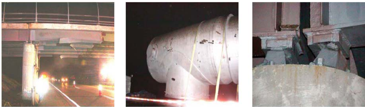
Figure 3-14: Impact to the Bridge 1021079 on Cleveland Drive in Buffalo, New York.
