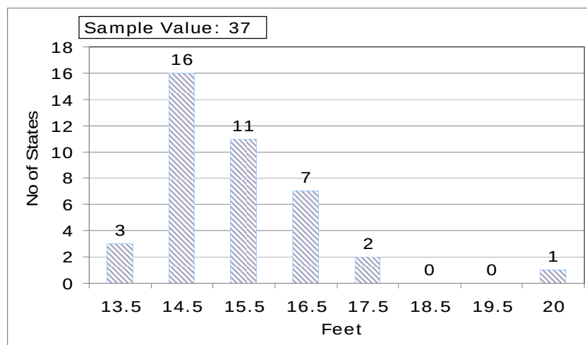
Figure 2-19: Bridge Vertical Under-Clearance Requiring Sign Posting
