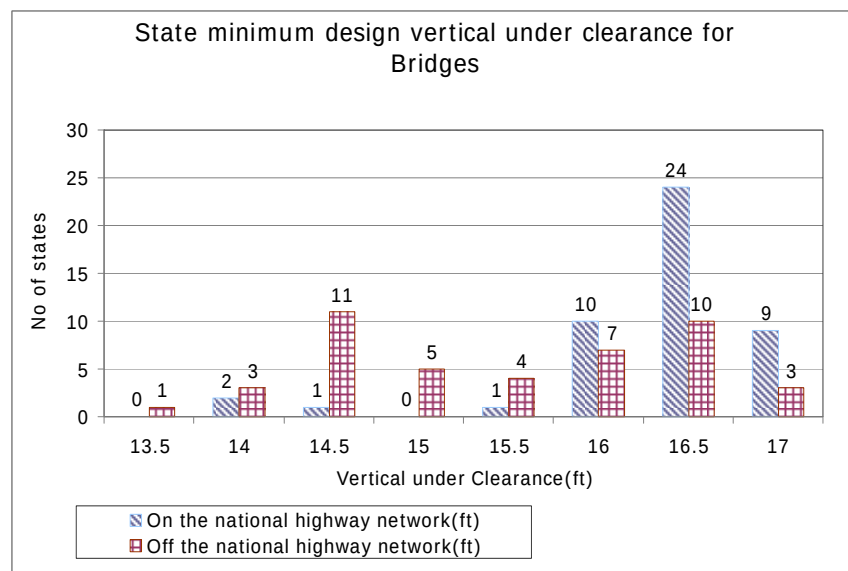
Figure 2-11: Minimum Design Vertical Under-Clearance.
