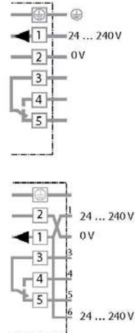
Connection diagramm
