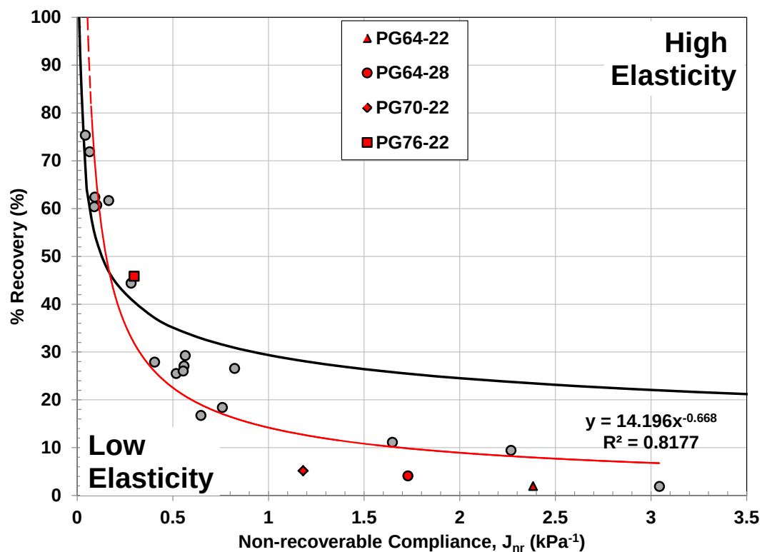
Figure 28 – J_{nr} - % Recovery Curve and Data for Binders Tested at 64°C
