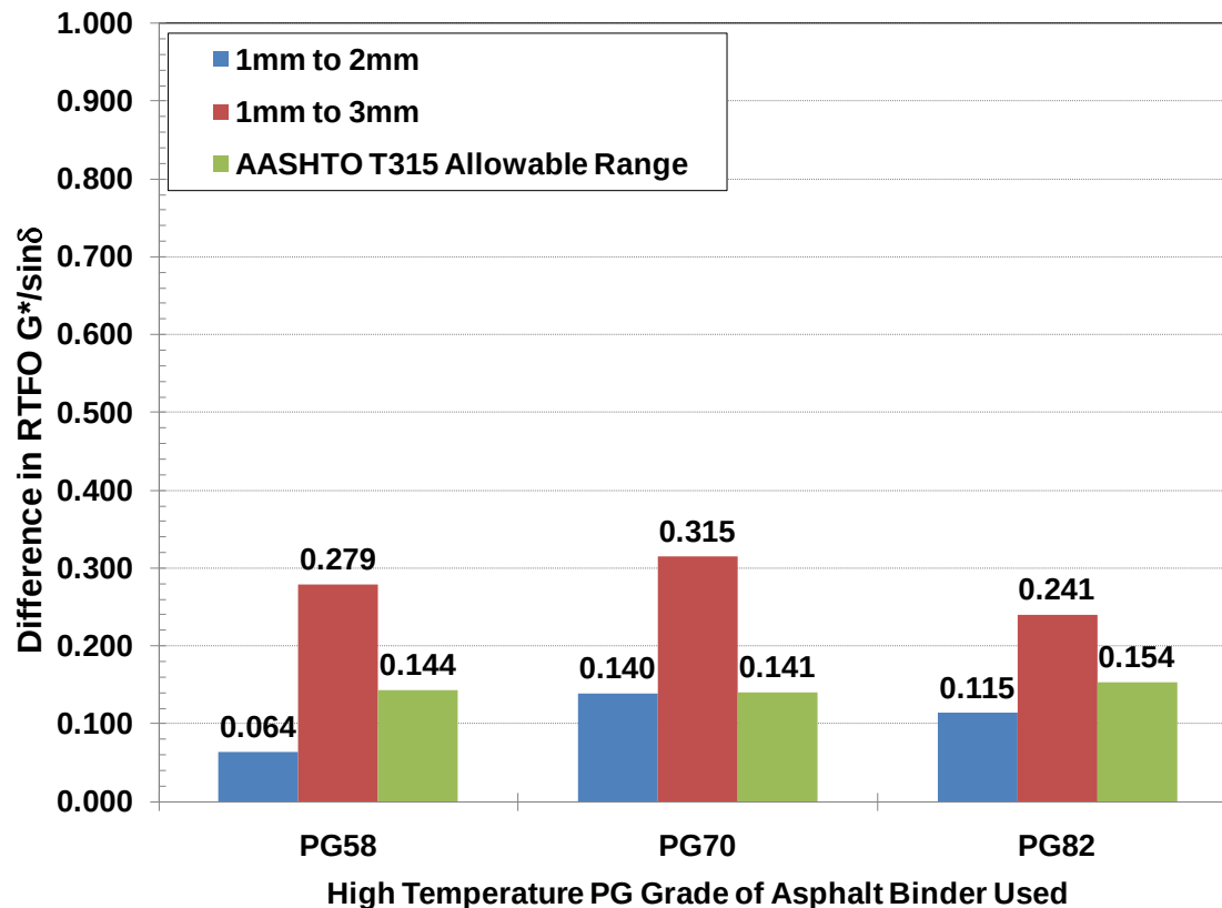
Figure 14 – Failure Temperature Results for RTFO Binder Condition
