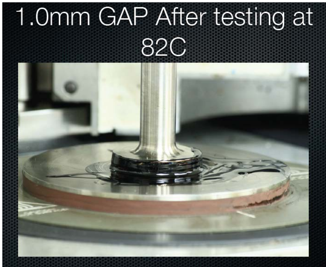
Figure 15 – 1.0mm Gap Height Immediately After Testing at 82°C
