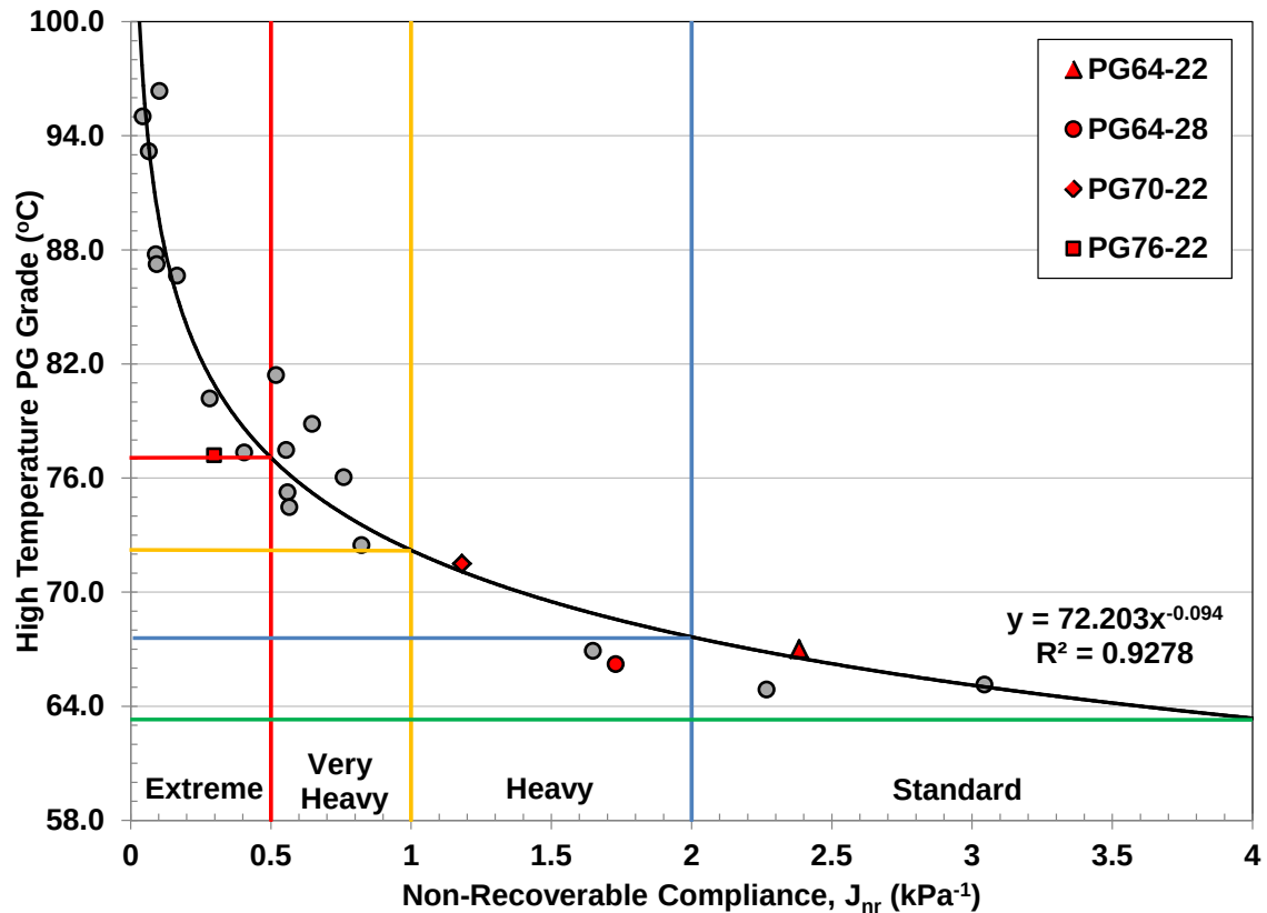
Figure 33 – High Temperature PG Grade with 1.0 mm Gap Height vs MSCR J_{nr} with 2.0 mm Gap Height at 64°C Test Temperature
