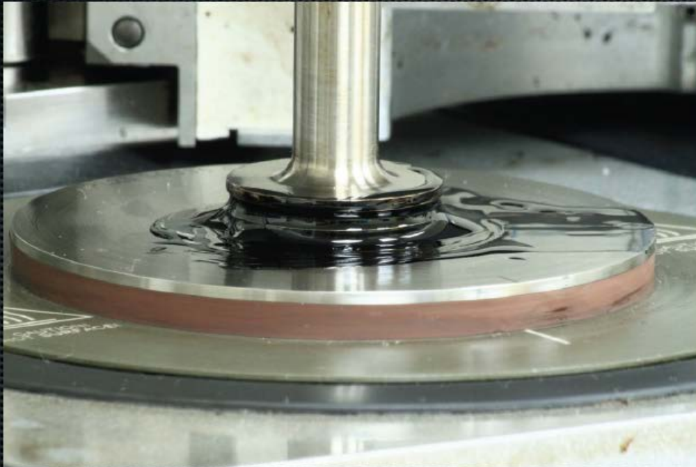
Figure 18 – 2.0mm Gap Height Immediately After Testing at 88°C
