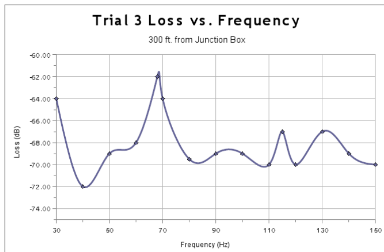
Figure 3: Loss vs. frequency for test at 300' from the manhole.
