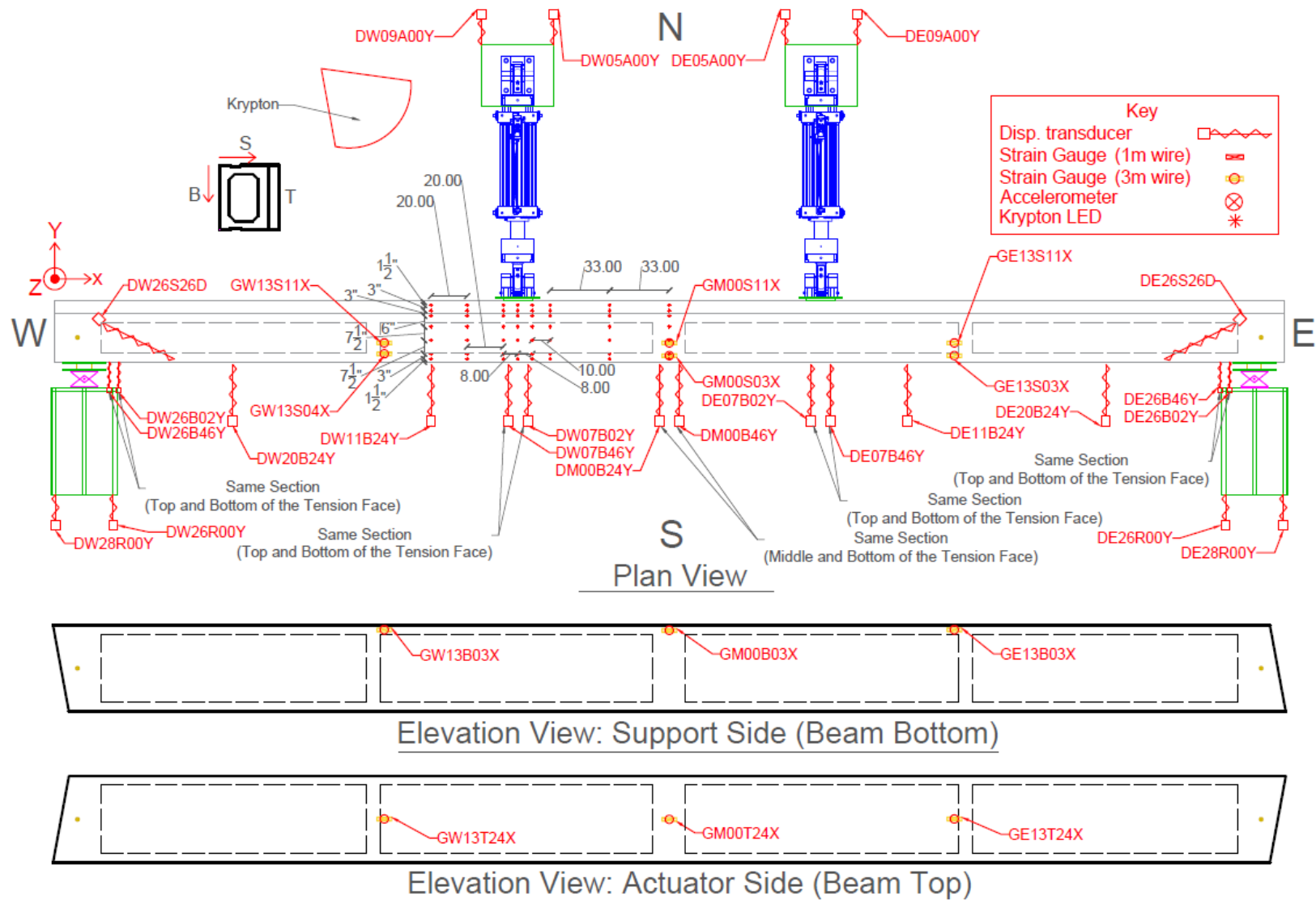
Figure 4-6 Beam 3 Instrumentation (service-level tests)
