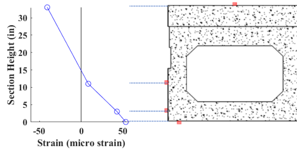
Figure 5-4 Strain profile at the peak force during the service-level test of unretrofitted Beam 1
