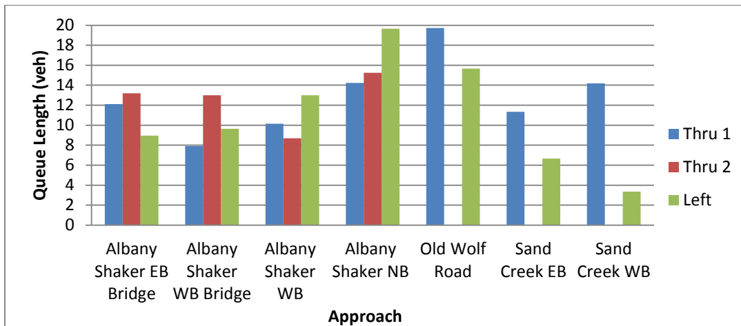
Figure 5.20: Queue lengths for weekday PM peak – after periods
