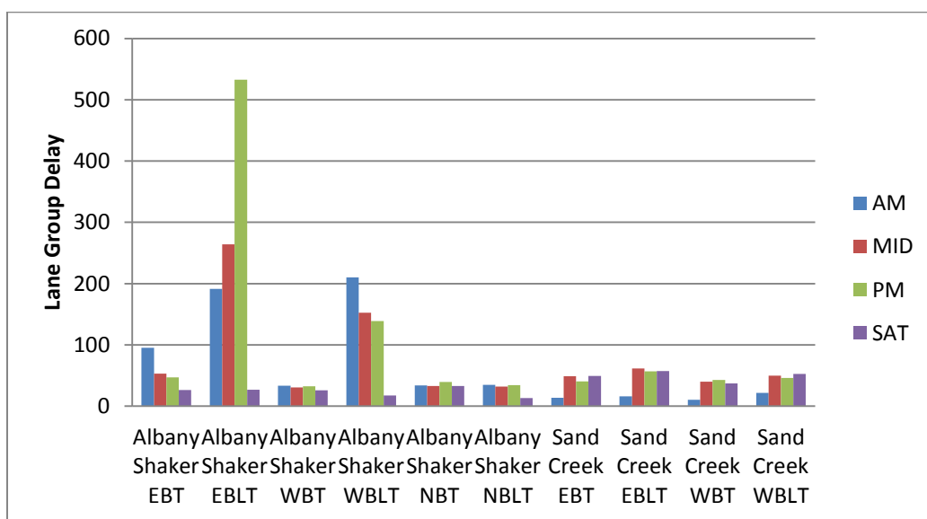
Figure 5.28: Average delay by lane group – after periods
