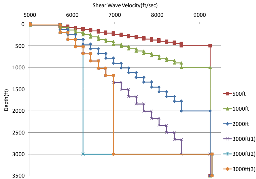
Fig. 1.9 Deep rock class A profiles analyzed
