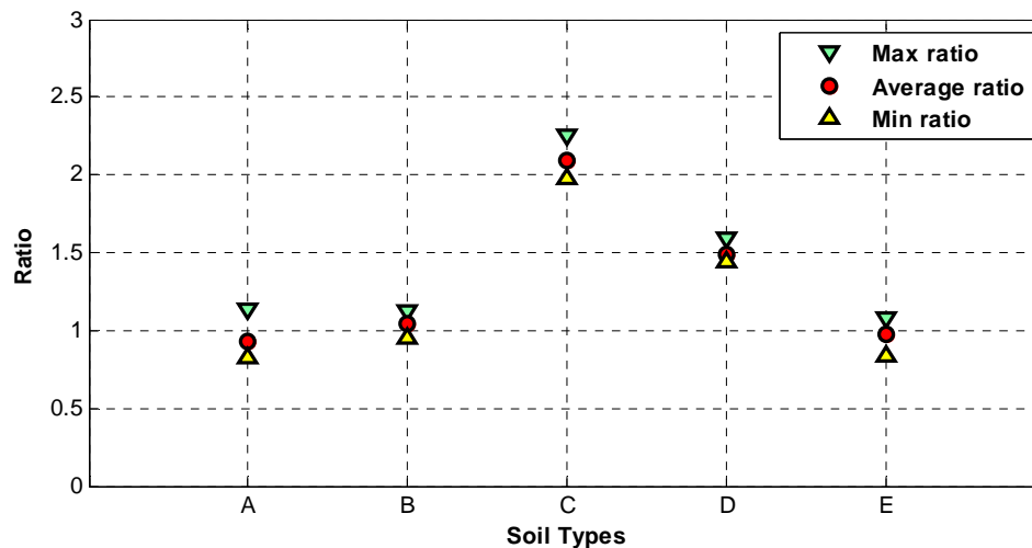
Fig. 2.20 Plot of range of ratios of response quantities using 1000 yr. NYCDOT and 1000 yr. AASHTO spectra for different soil types
