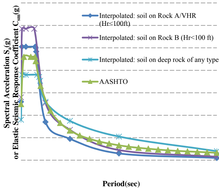
Fig. 1.2 Comparison of horizontal response spectra of 1000-yr return period: site class E.
