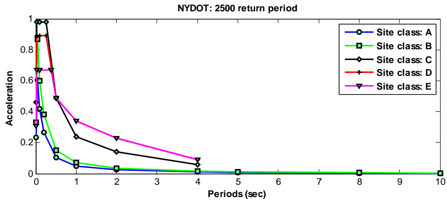
Fig. 2.18 Design spectra: NYCDOT 2500 yr. return period
