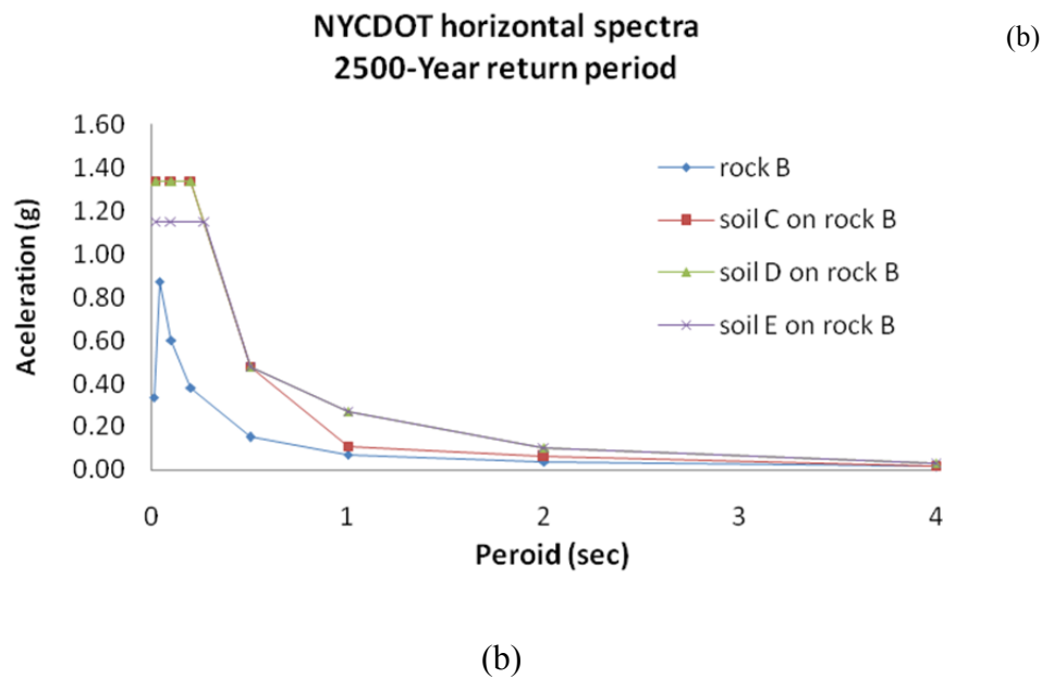
Fig. 1.4 Comparison of response design spectra of rock and soil sites for the 2500-year earthquake: (a): rock class A and soil on rock class A; (b) rock class B and soil on rock class B.
