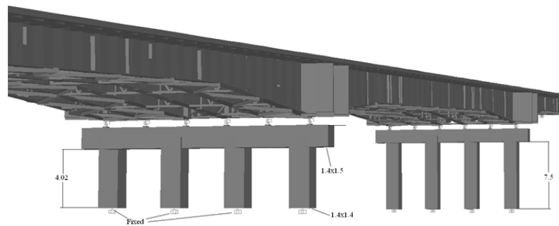
Fig. 2.12 Details of the substructure
