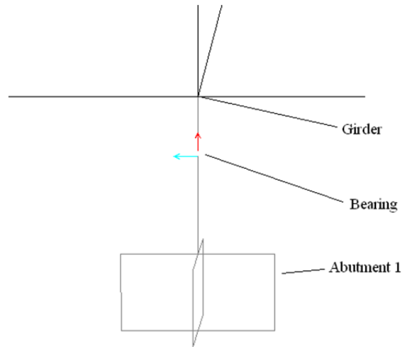
Fig 2.11 Nonlinear link element for modeling of bearings
