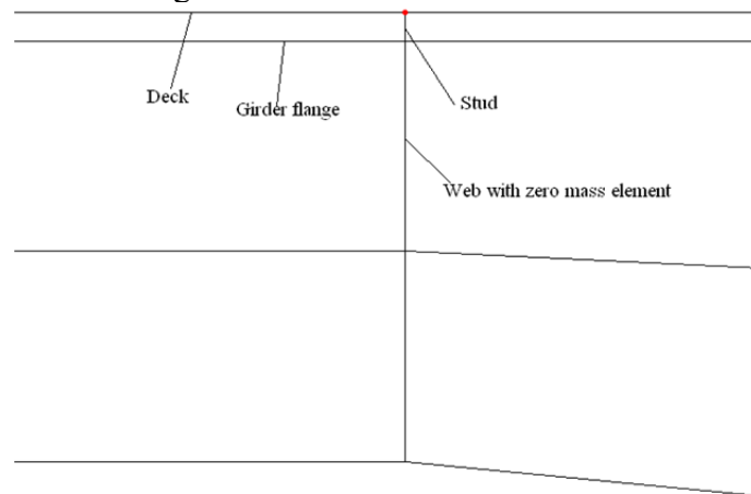
Fig. 2.6 Modeling of studs in the bridge deck
