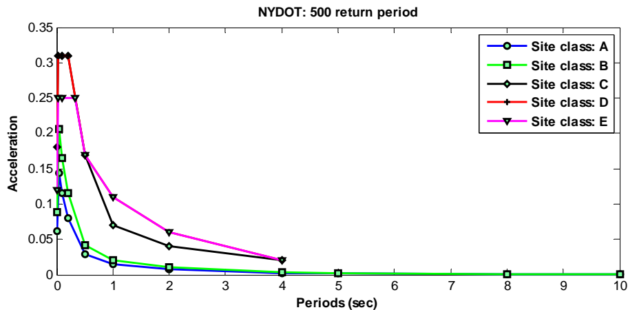
Fig. 2.15 Design spectra: NYCDOT 500 yr. return period
