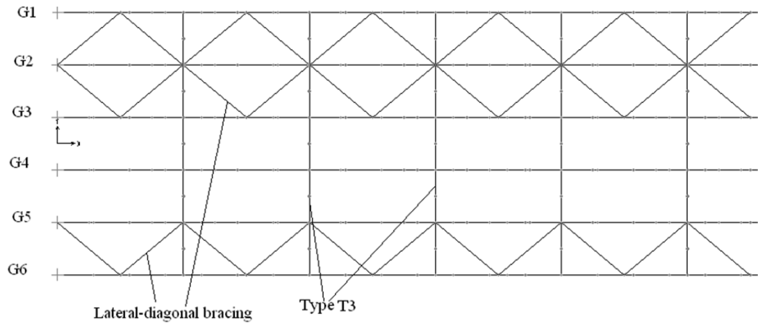
Fig. 2.9 The layout of the lateral-diagonal bracing at the bottom flange of the I-shape girder
