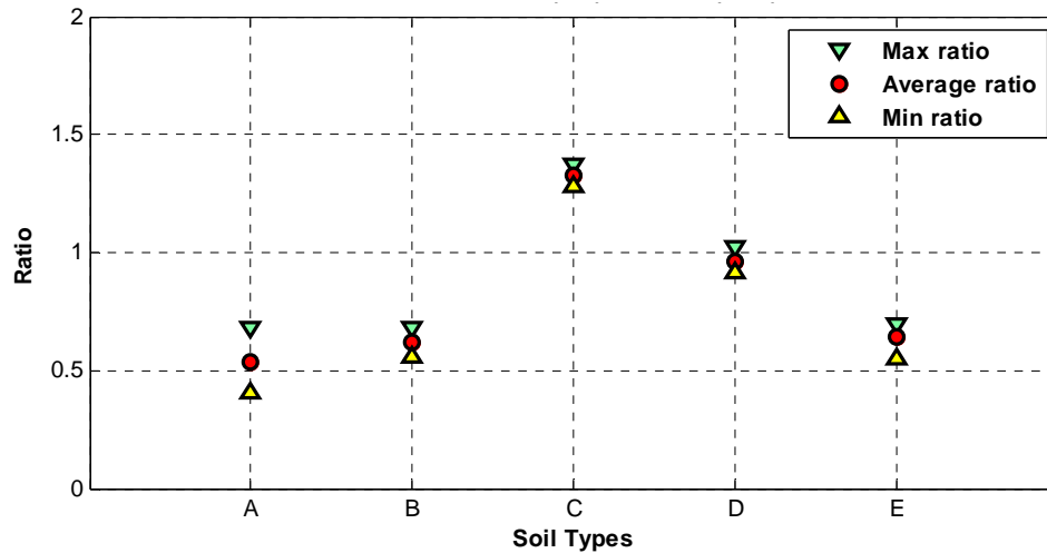
Fig. 2.21 Plot of range of ratios of response quantities using 500 yr. NYCDOT and 1000 yr. AASHTO spectra for different soil types
