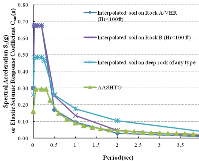
Fig. 1.1 Comparison of horizontal response spectra of 1000-yr return period: site class D
