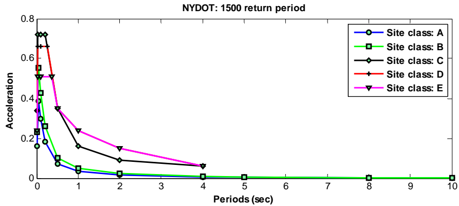
Fig. 2.17 Design spectra: NYCDOT 1500 yr. return period
