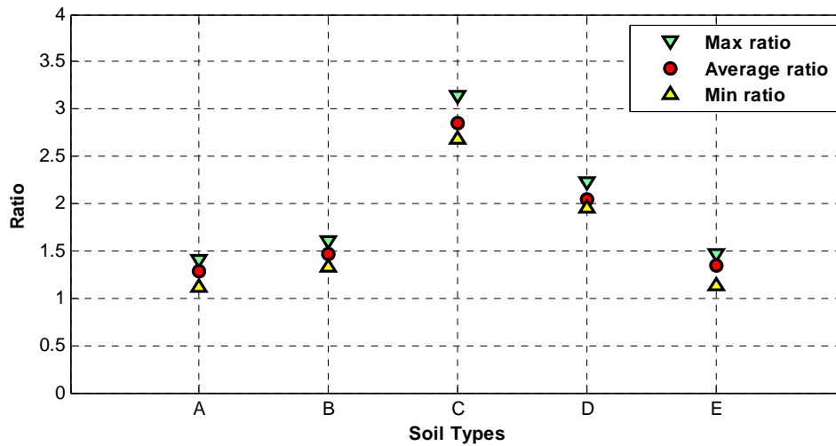
Fig. 2.19 Plot of range of ratios of response quantities using 1500 yr. NYCDOT and 1000 yr. AASHTO spectra for different soil types
