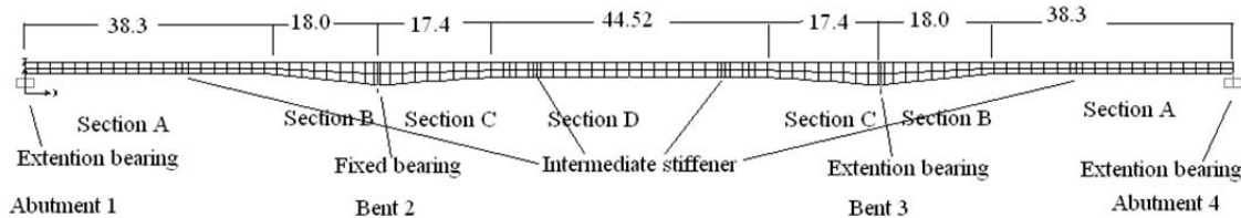
Fig. 2.7 Intermediate stiffeners I the longitudinal girders
