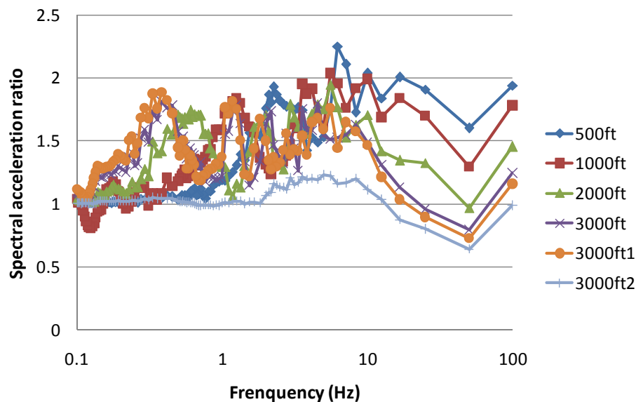
Fig. 1.8 Spectral acceleration ratio for the rock class B profiles analyzed (2500-year earthquake)
