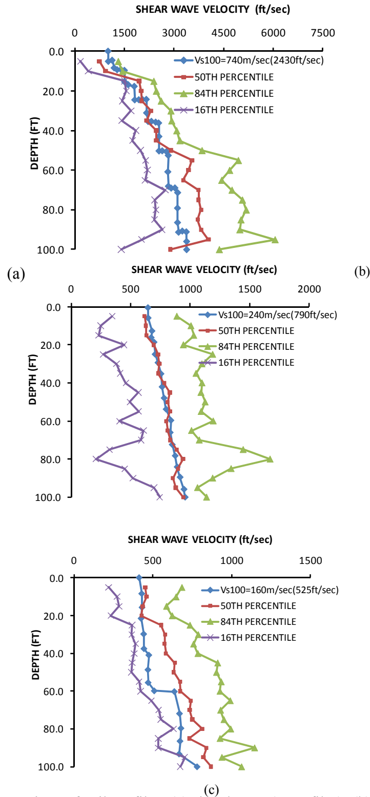
Fig. 1.11 Comparison of soil profiles: (a) site class C (7 profiles); (b) soil class D (34 profiles); (c) soil class E (24 profiles)
