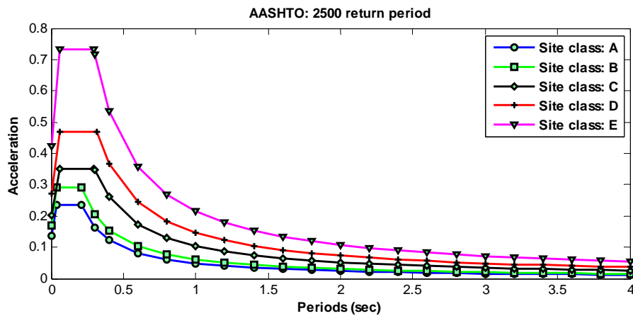
Fig. 2.14 Design spectra: USGS 2500 yr. return period
