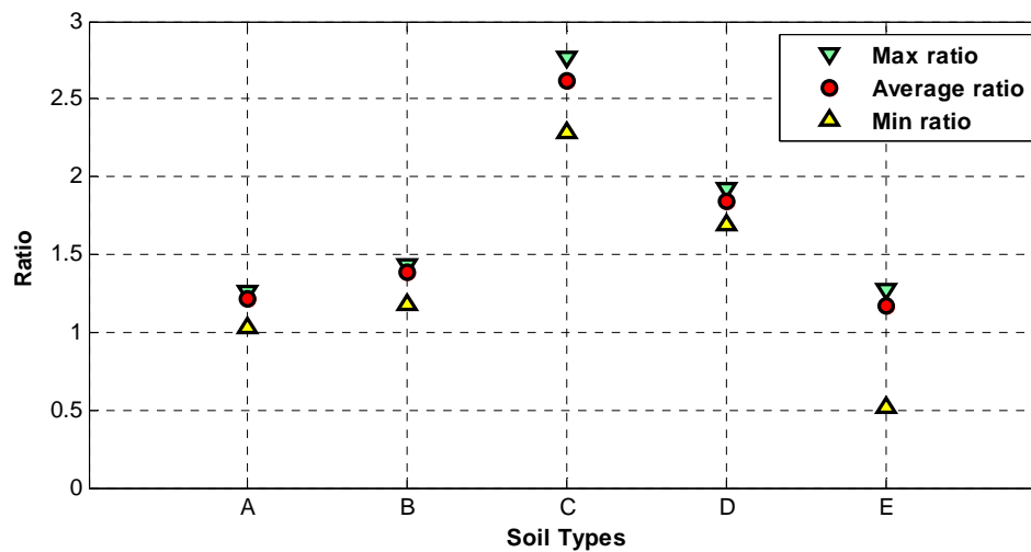
Fig. 2.22 Plot of range of ratios of response quantities using 2500 yr. NYCDOT and 2500 USGS spectra for different soil types
