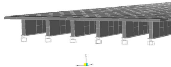
(b) 3-D Bridge Deck Model
