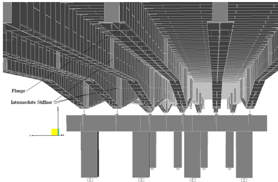
Fig. 2.4 3-D view of underside of the bridge
