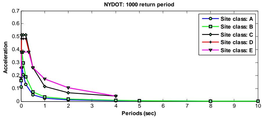
Fig. 2.16 Design spectra: NYCDOT 1000 yr. return period (based on interpolation)
