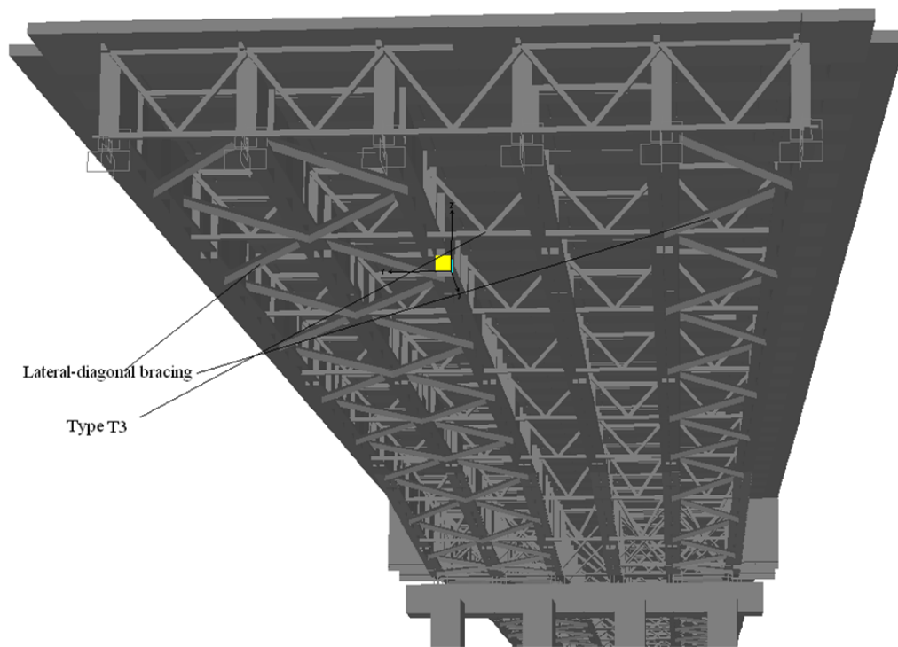
Fig. 2.10 Layout of lateral-diagonal bracing in the superstructure of the bridge
