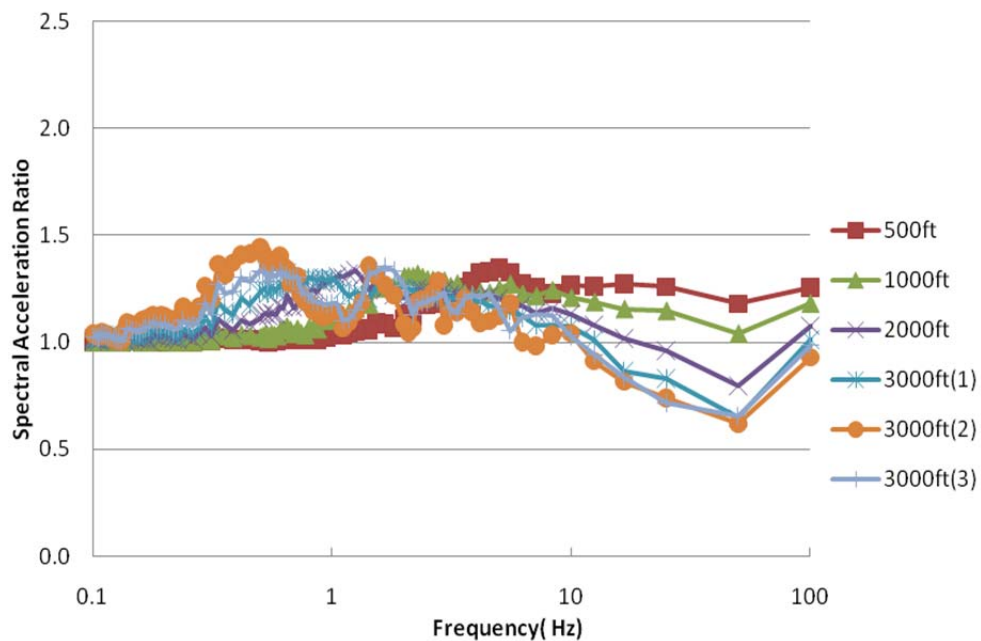
Fig. 1.9 Deep rock class A profiles analyzed
