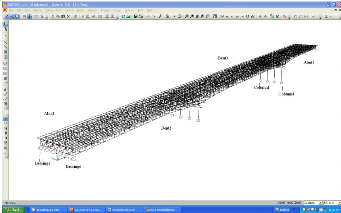
Fig. 2.2 Whole bridge 3-D finite element model using SAP2000
