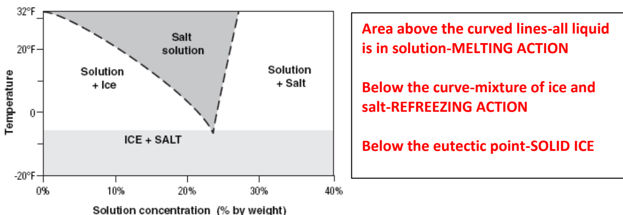
Figure 7.1: Phase Diagram of Salt
