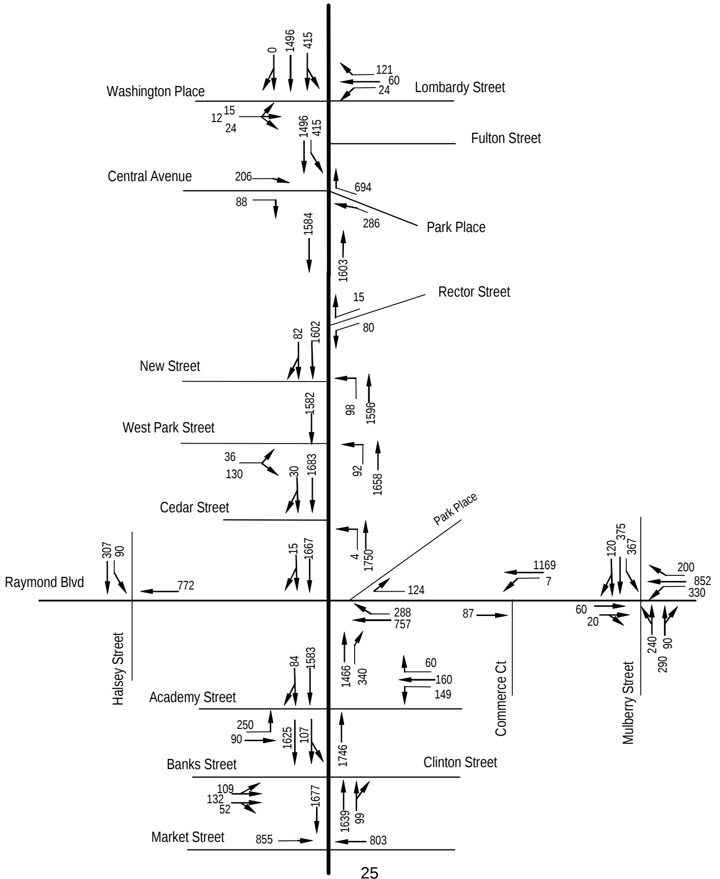
Figure 3. PM Peak Hour Volumes Broad Street – Volume Diagram (PM Peak)
