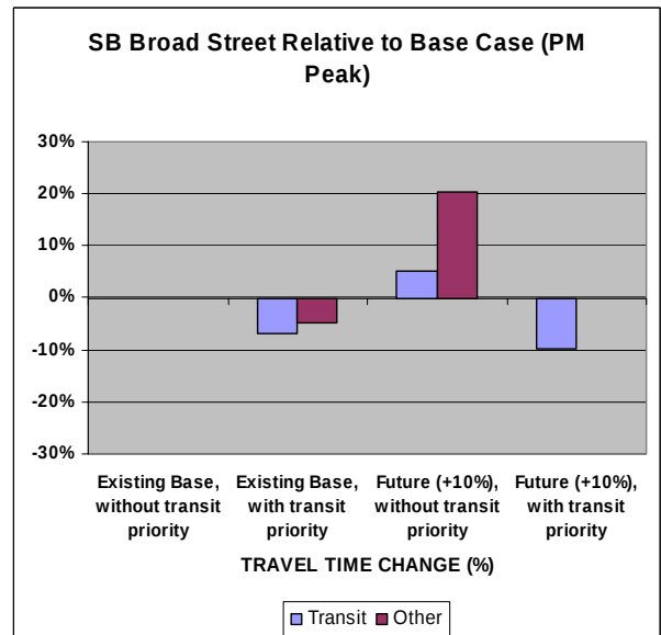
Figure 6. Impact of Broad Street Transit Priority on Broad Street Transit and Auto
