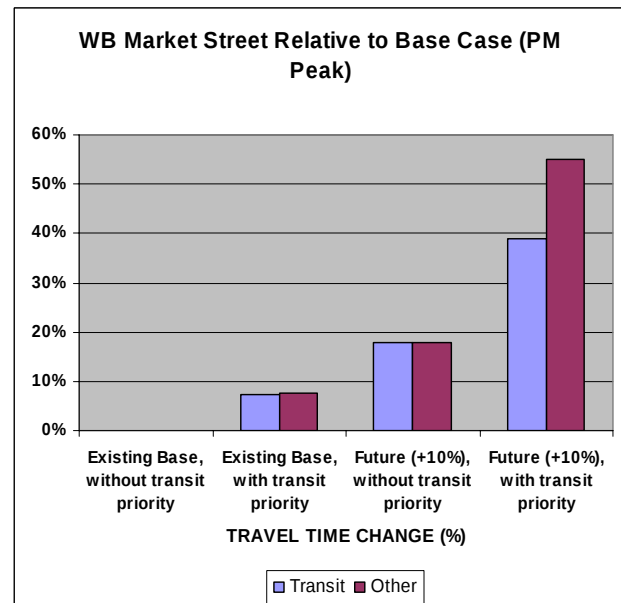
Figure 8. Impact of Broad Street Transit Priority on Market Street Traffic
