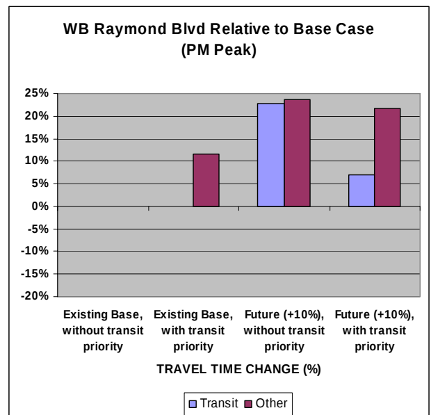
Figure 7. Impact of Broad Street Transit Priority on Raymond Blvd Traffic
