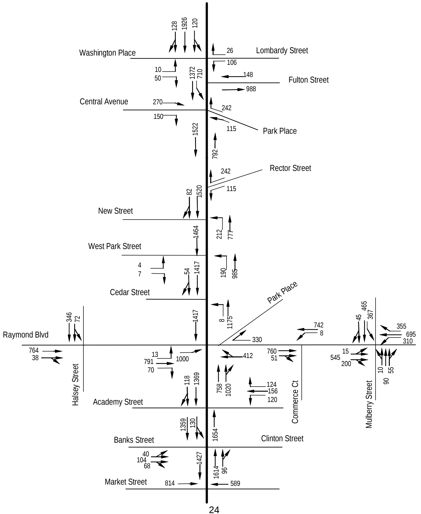
Figure 2. AM Peak Hour Volumes Broad Street – Volume Diagram (AM Peak)
